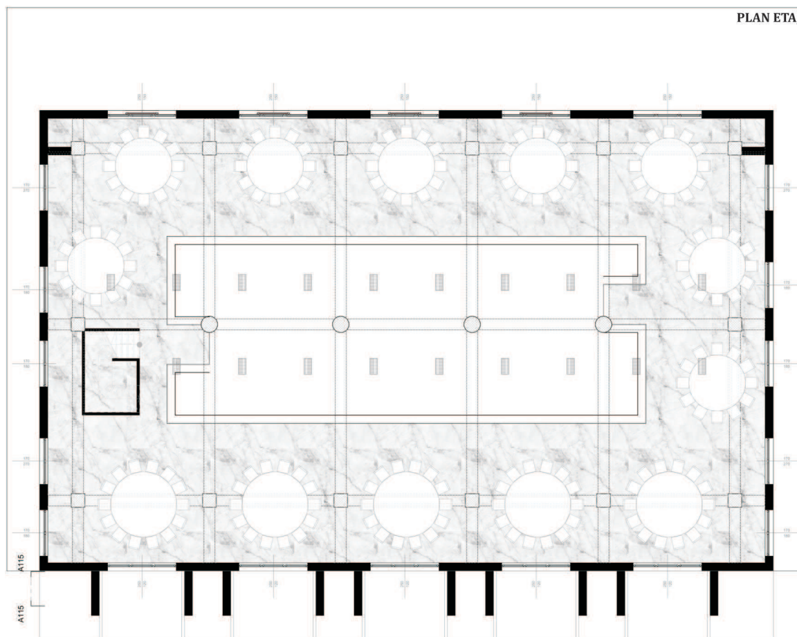
PLAN PARTER
