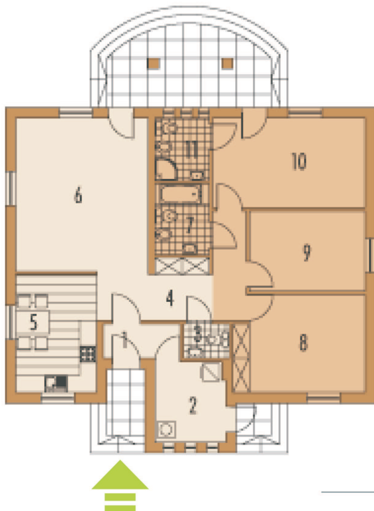
Plan PARTER
