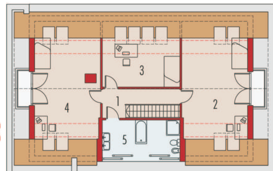
Plan MANSARDĂ
