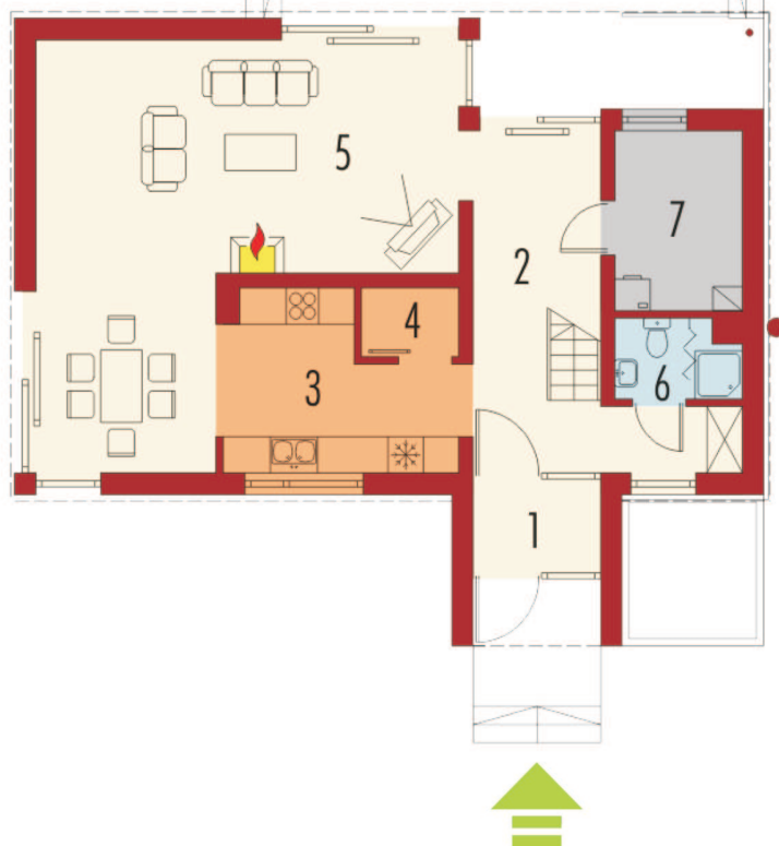
Plan PARTER
