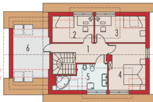
Plan MANSARDĂ
