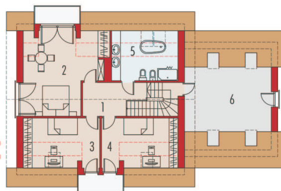
Plan MANSARDĂ
