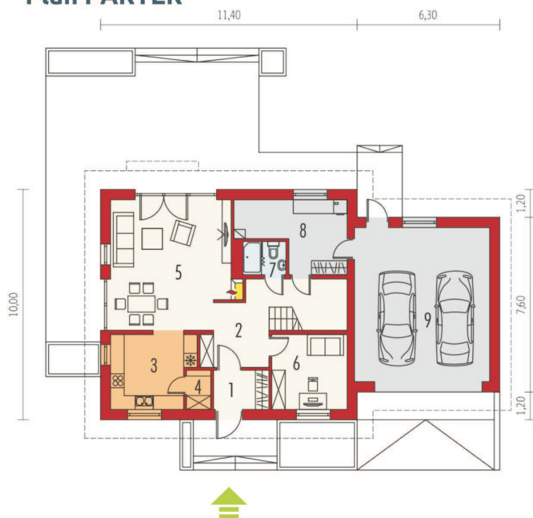
Plan PARTER
